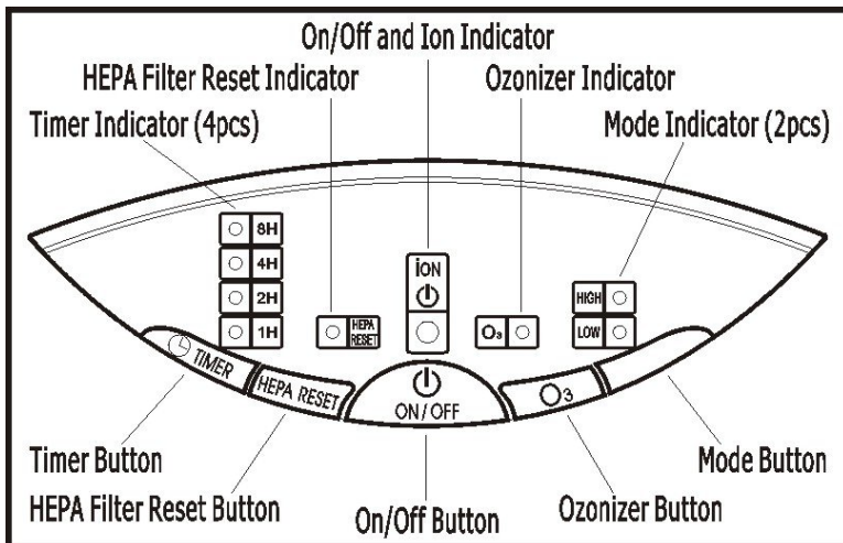
Figure 1-2 (For 9079C)
