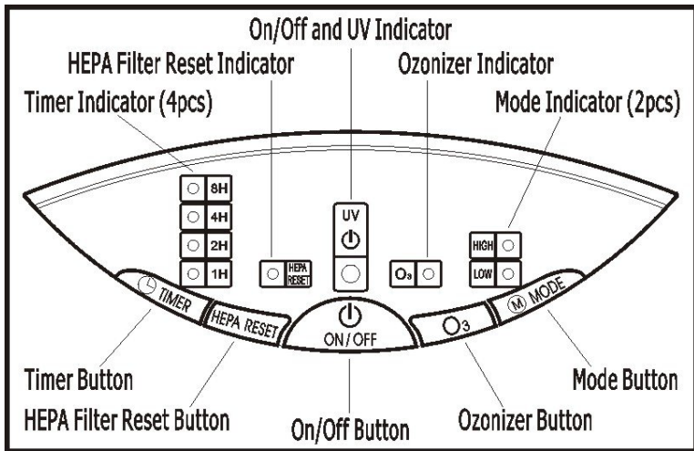
Figure 1-3 (For 9079D)
